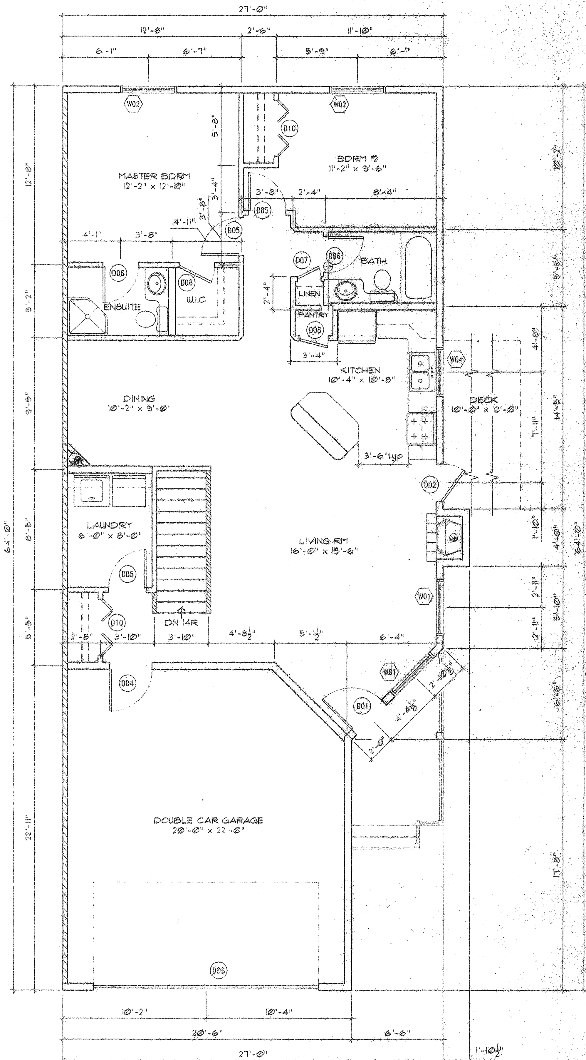
MAIN FLOOR PLAN (UNIT #2) 1136 SQ. FT. SCALE: 1/4" = 1'-0"
